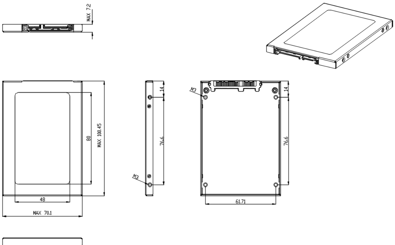
Figure 2-1 Product Dimensions
